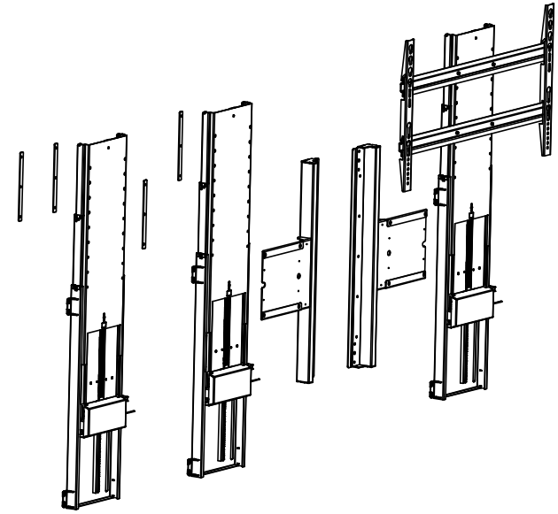
EXPLODED
